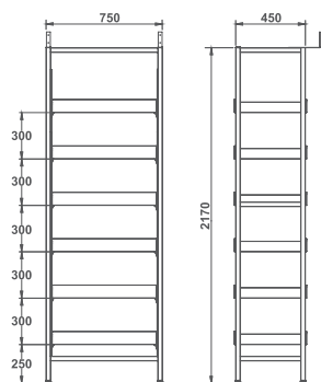
ESTANTE MODULAR WALK IN COOLER
