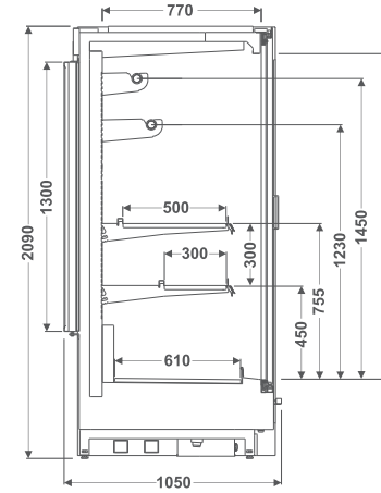
EVTVPT Expositor Vertical Vision Pass Through
